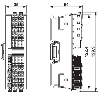
Dimensional drawing
