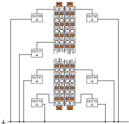
Connection in 1-conductor technology
