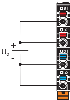
Parallel supply of the supply voltage
